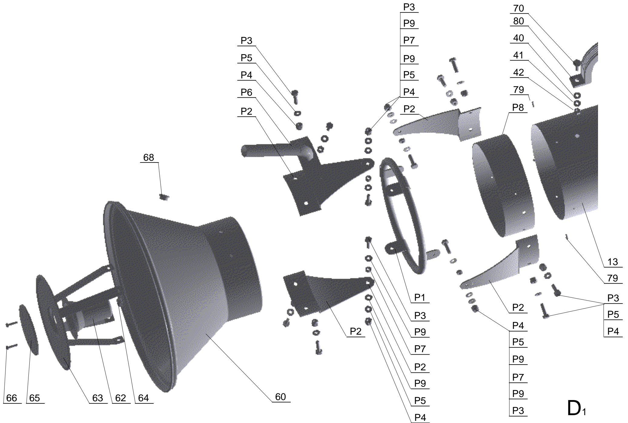
Snorkvac™ Fume Extractor Arm Drawing D1(Hood Assembly, 6 and 8 inch) Bench Mount
