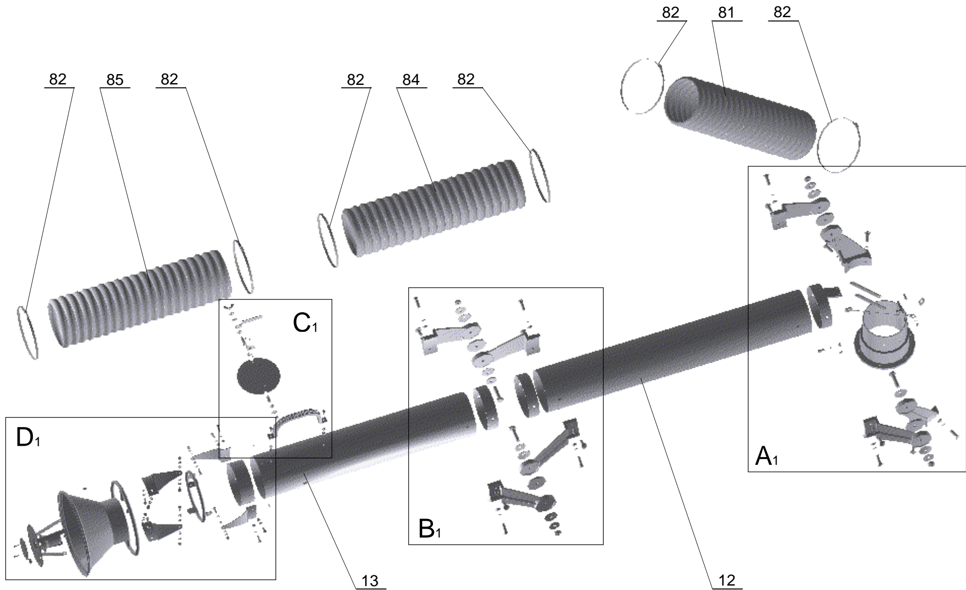
103 Snorkvac™ Fume Extractor Arm Drawing A1, B1, C1, D1 (All Assemblies, 6 and 8 inch) Bench Mount
